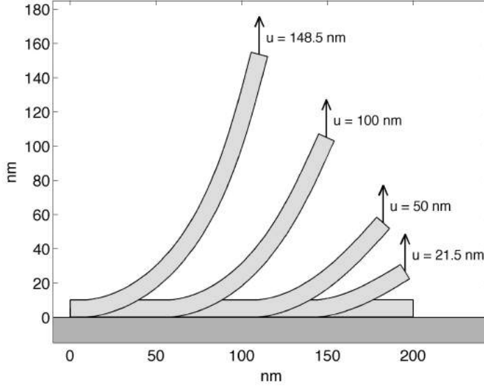
Figure 7: Strip deformation during peeling for the displacements u = 0 , u = 21.5 nm (which is the location of the maximum peeling force), u = 50 nm, u = 100 nm and u = 148.5 nm. The strip parameters are taken as E = 2 GPa, h = 10 nm, A_H = 10^{-19} J and r_0 = 0.4 nm.
