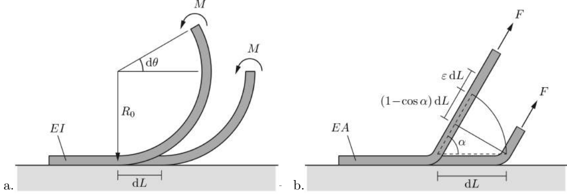
Figure 1: Fundamental peeling examples: a. peeling by pure bending; b. peeling by pure stretching.
