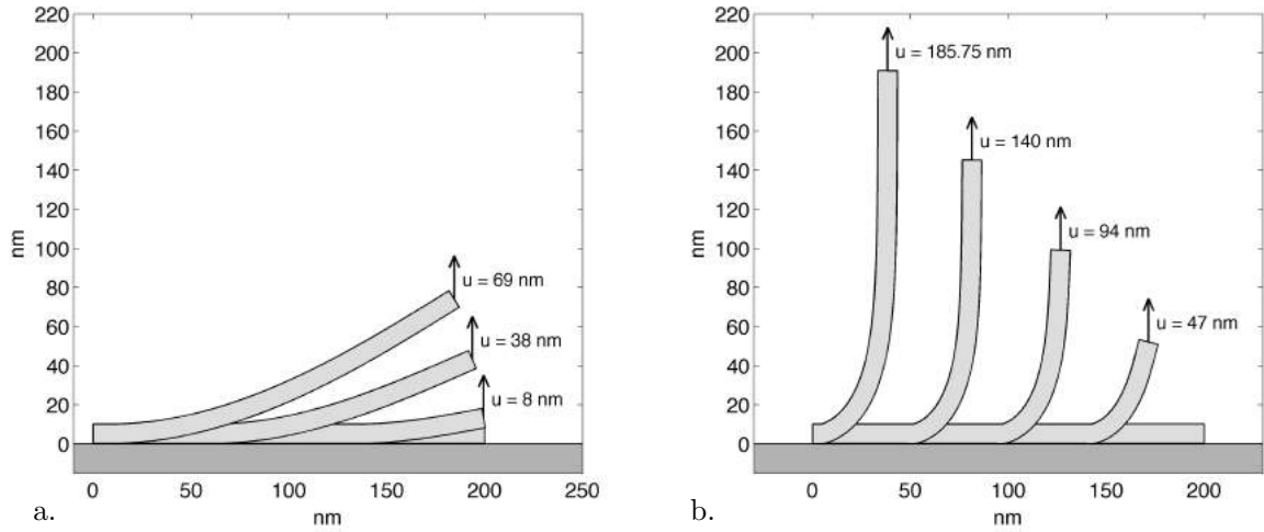
Figure 9: Peeling deformations of (a.) the stiff strip ( E/A_H = 10E_0/A_{H0} ) and (b.) the soft strip ( A_H/E = 10A_{H0}/E_0 ).
